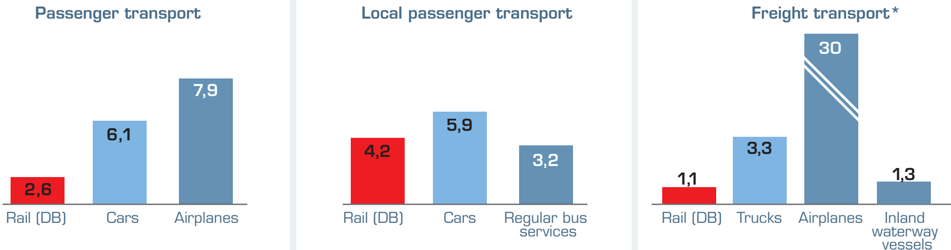
Consumption of primary energy in litres of fuel per 100 passenger kilometres (freight transport: litres of Diesel per 100 ton kilometres); data basis 2008, *referred to Europe
